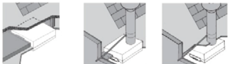
Ceiling mounting with flat ducting
